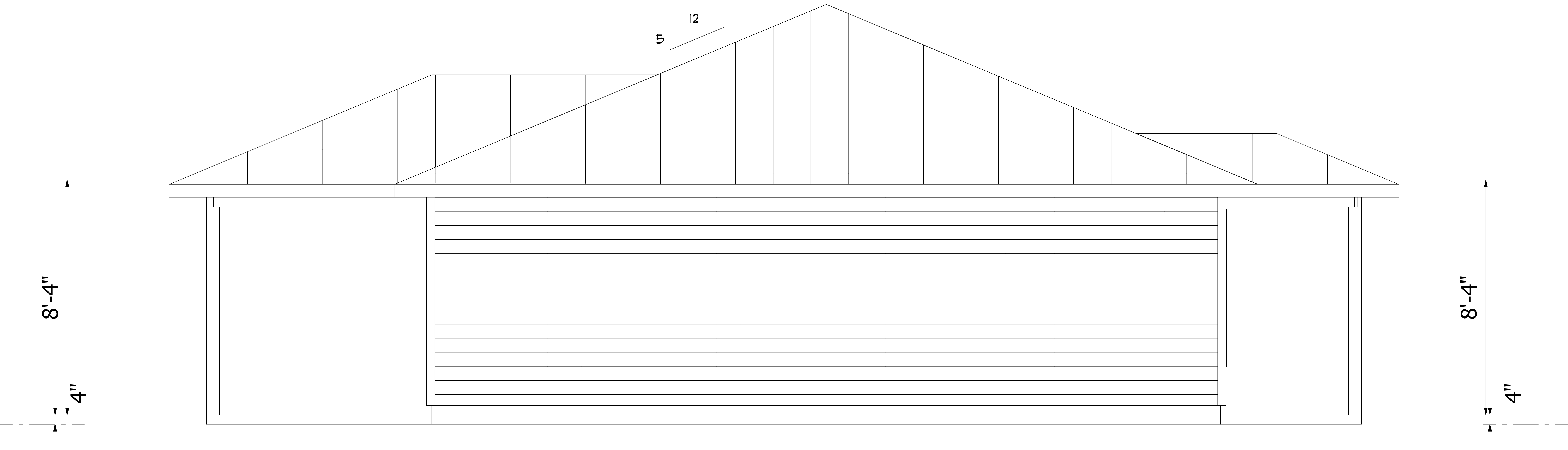
LEFT ELEVATION
